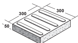
300x300x50 Tactile Paver Directional
