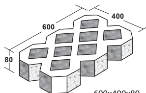
600x400x80 Turf Block
